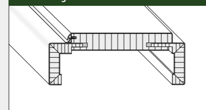
smart 2 -Zarge B60
