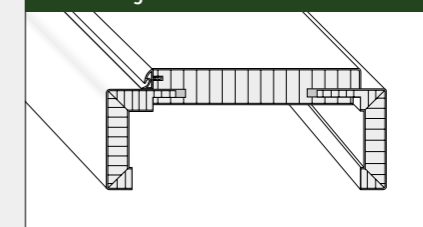
smart 2 -Zarge B80
