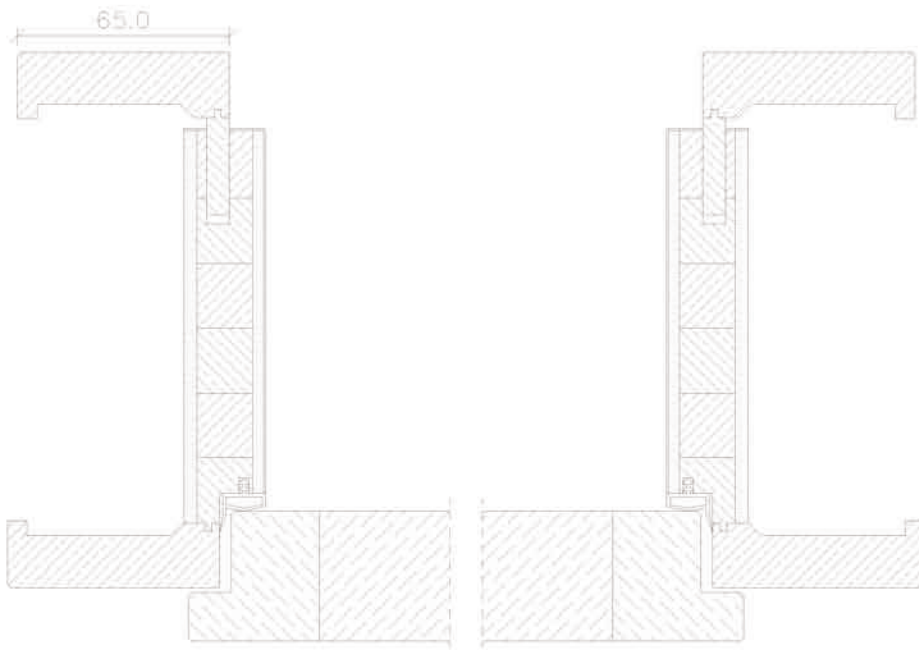
Zarge MZ-I
