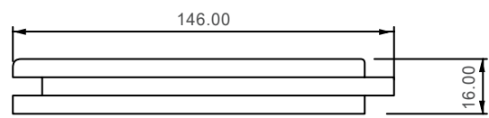
Swingprofil - Short
